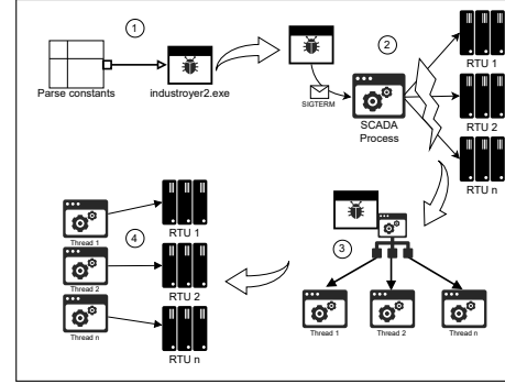
(e) Industroyer 2 payload
