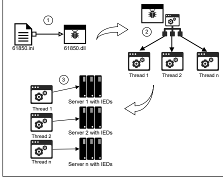
(a) IEC-61850 payload
