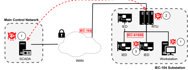
Figure 13: Attack surfaces.
