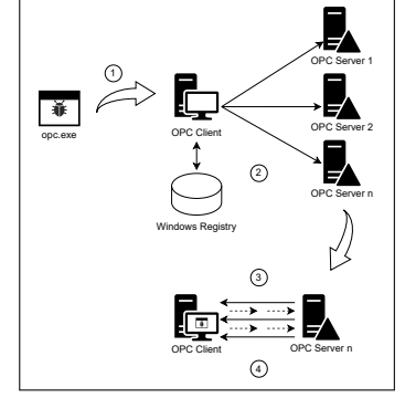
(c) OPC-DA payload
